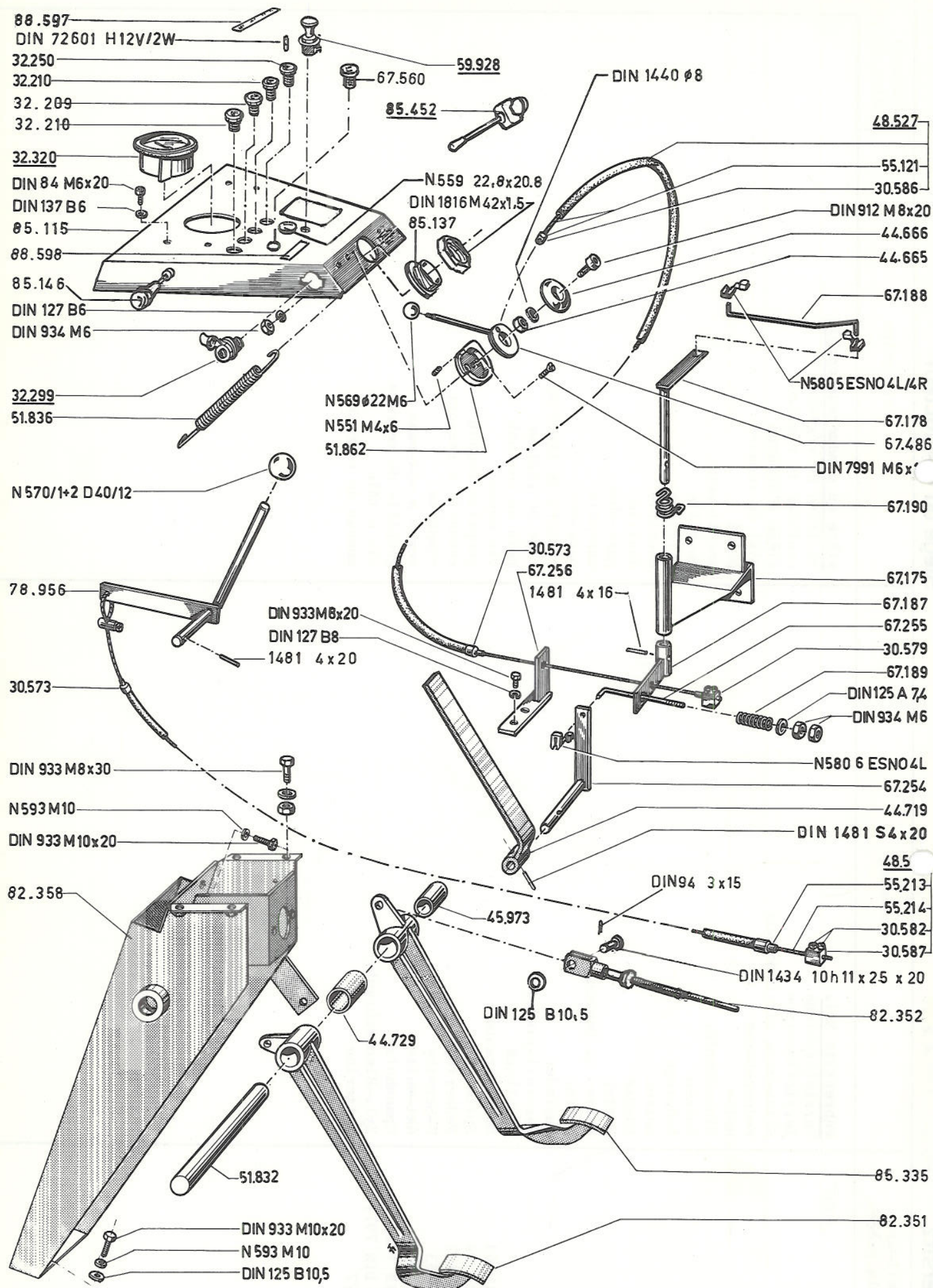
Armaturenbrett, Pedalsupport
